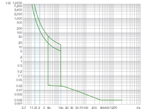
J Frame 175 - 250 Amp
