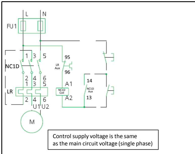
Single Phase - Wiring Diagram
