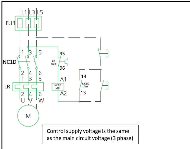
Three Phase - Wiring Diagram
